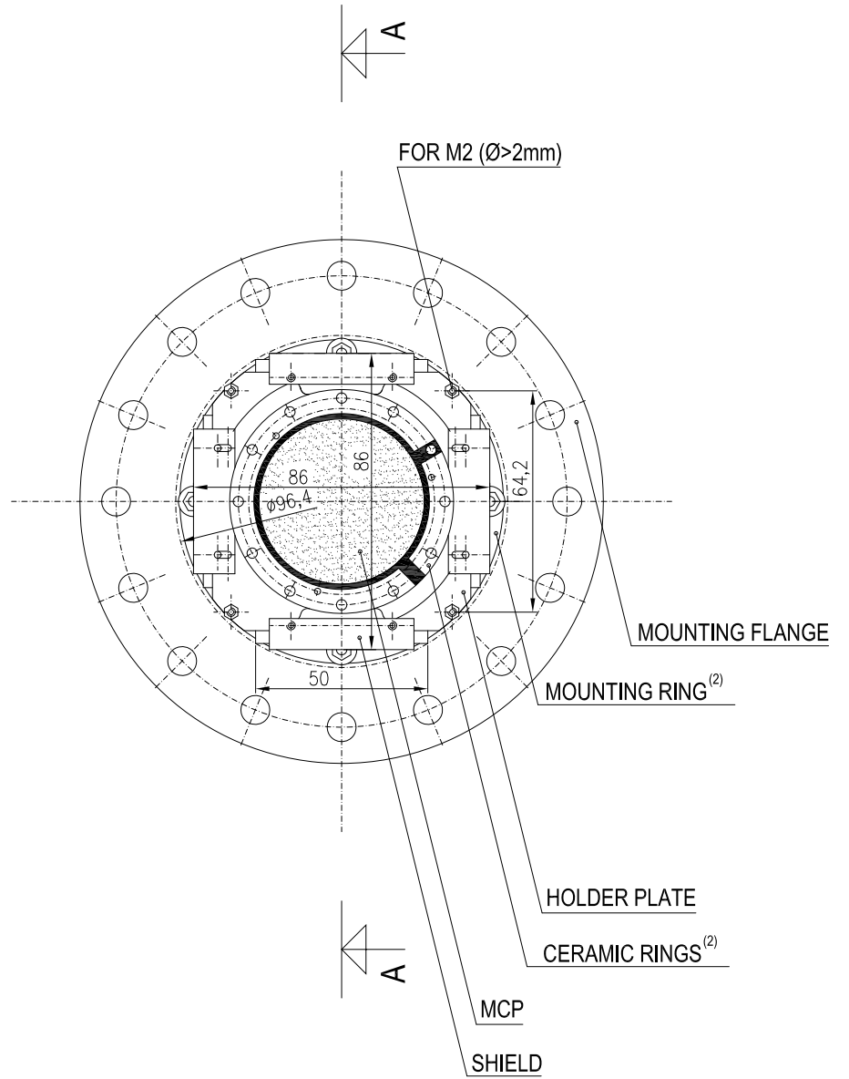
TOP VIEW
