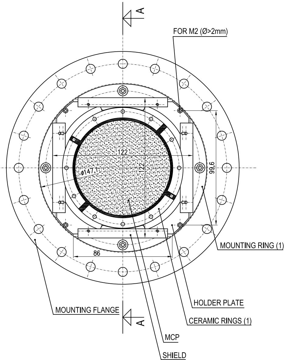
TOP VIEW
