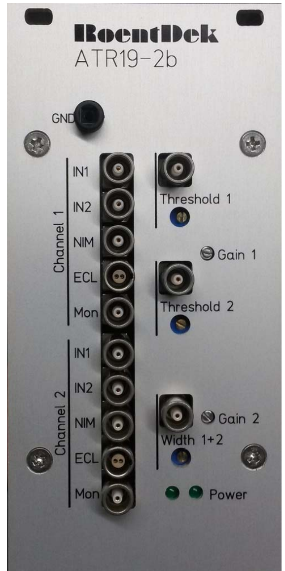
Front panel of the RoentDek ATR19-2(b) module
