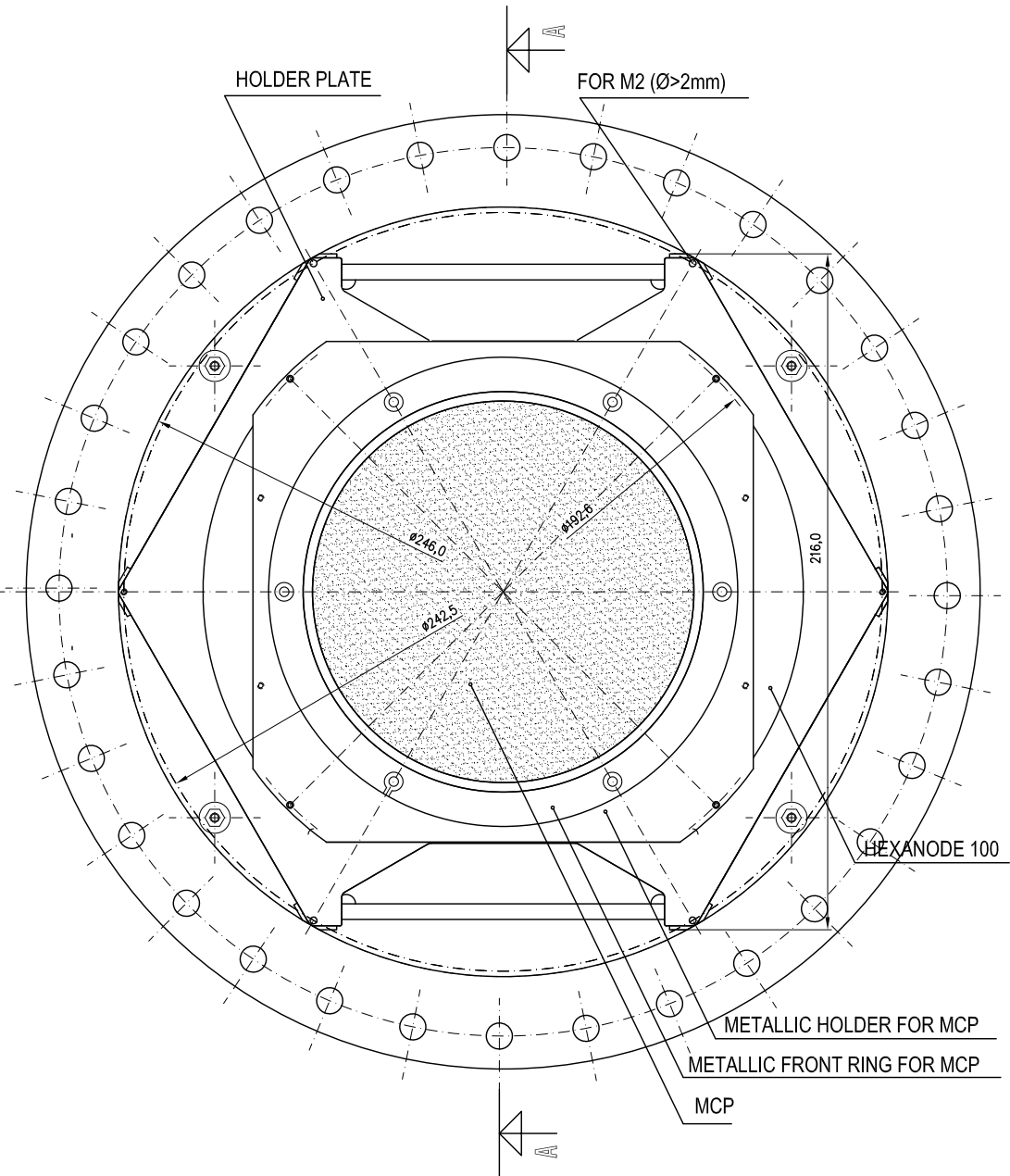
TOP VIEW
